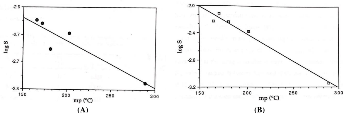
Figure 1: The relationship between the observed water solubility (A) and phosphate buffer solubility (B) in mole fraction (log S) and melting points of NSAIDs studied.
